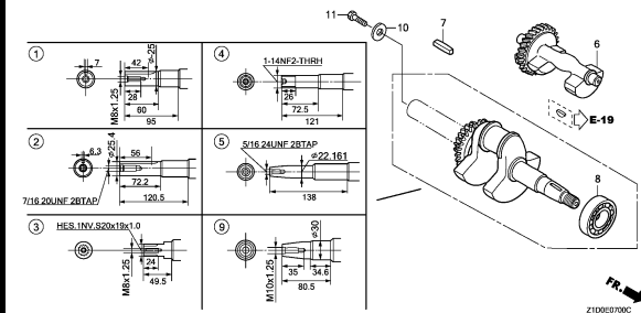
CRANKSHAFT
