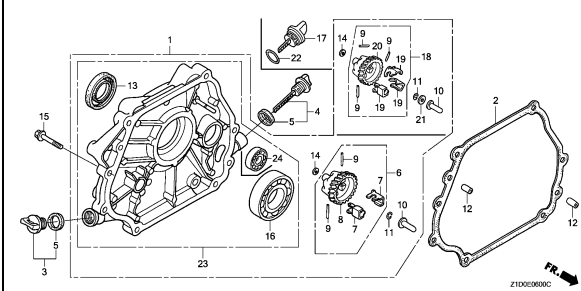
CRANKCASE COVER(4)
