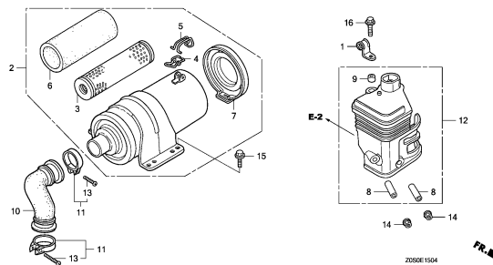
AIR CLEANER(RAMMER)
