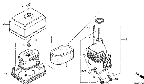
AIR CLEANER(GENERATOR)
