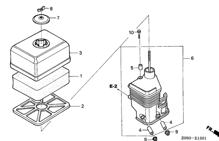
AIR CLEANER(RAMMER)
