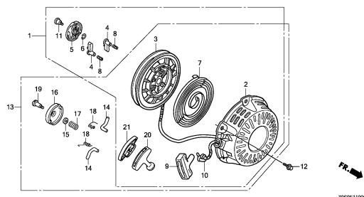
RECOIL STARTER(1)
